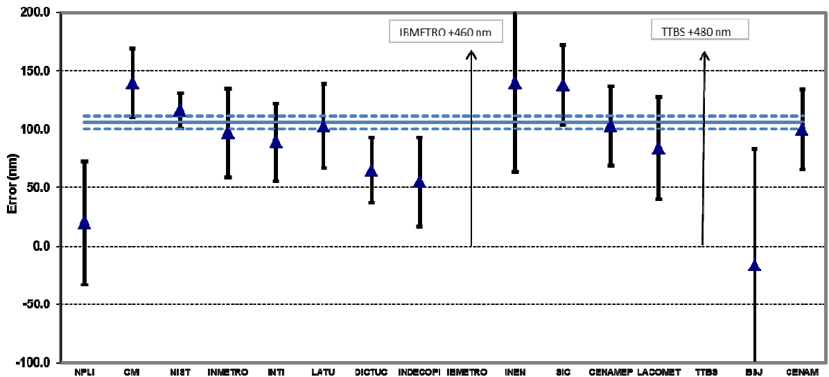
Graph 28. Ceramic gauge block, nominal length 50 mm ( 011002 )
