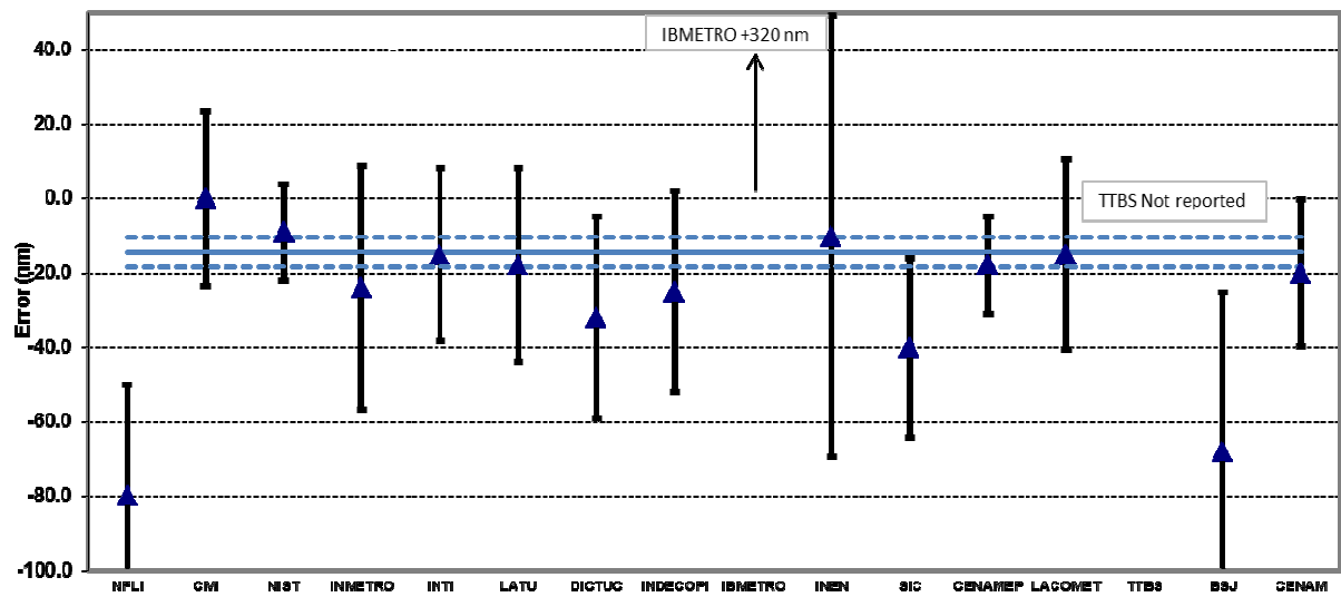
Graph 27. Ceramic gauge block, nominal length 10 mm ( 052351 )
