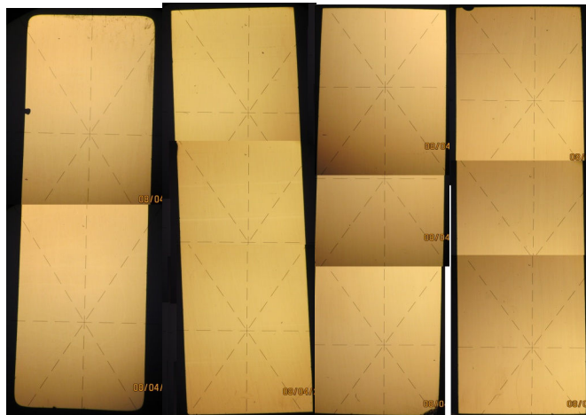
Figures 8, 9, 10 and 11. Aspect of the measuring faces of the 10, 50, 75 and 100 mm Ceramic GB at the end of circulation.
