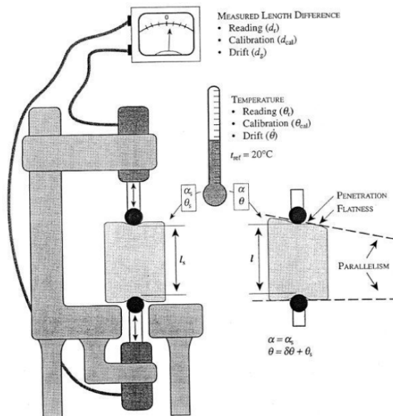
Figure 1. Illustration of the calibration method of GB by mechanical comparison showing the different variables of influence (taken from [8]).
