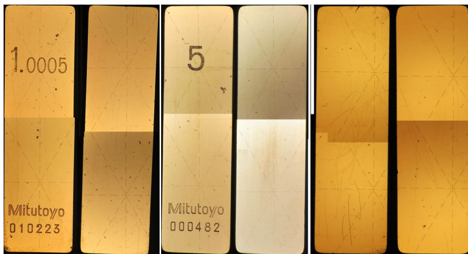
Figures 1, 2 and 3. Aspect of the measuring faces of the 1.000 5, 5 and 7 mm Steel GB at the end of circulation.
